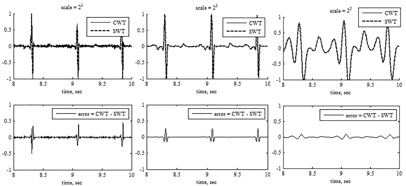
Fig. 2. Wavelet transforms and their error at scale 2^1, 2^3, 2^5 .
