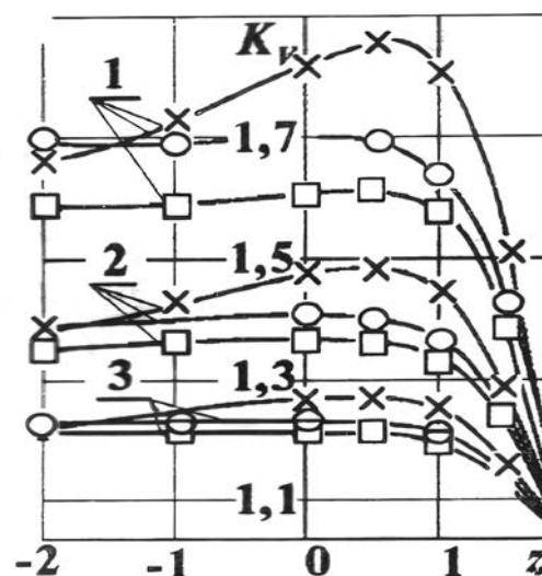
Fig. 2. Change in the K_v simplex along the z axis: 1 – Pe = 77.75 ; 2 – Pe = 116.625 ; 3 – Pe = 155.5 ; —□— the “five-layer coating — sublayer — base” system with constant spraying productivity; —×— the “five-layer coating — sublayer — base” system with constant coating thickness \Delta_{3c} = 0.0255 ; —○— separate steel base
