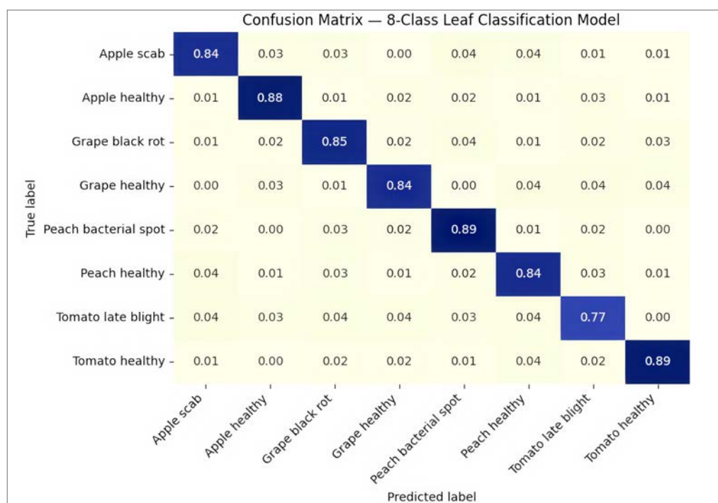
Fig. 12. Normalized confusion matrix for eight leaf classes. Dark diagonal cells indicate correct classifications, while lighter off-diagonal regions show minor confusion between visually similar categories
