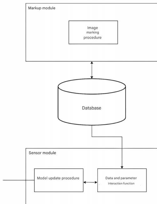
Fig. 7. Continuation of the functional scheme
