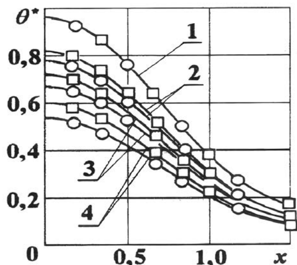
Fig. 1. Dependence \theta^* = f(x) – for y = 0, z = -0.513 in the layered heterogeneous system “five-layer coating-sublayer-base”: 1 – Pe = 77.75 ; 2 – Pe = 116.625 ; 3 – Pe = 155.5 ; 4 – Pe = 233.25 ; —□— constant spraying productivity; —○— constancy of coating thickness \Delta_{3c} = 0.0255
