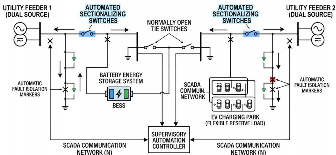
Fig. 3. Self-Healing Smart Distribution Grid
