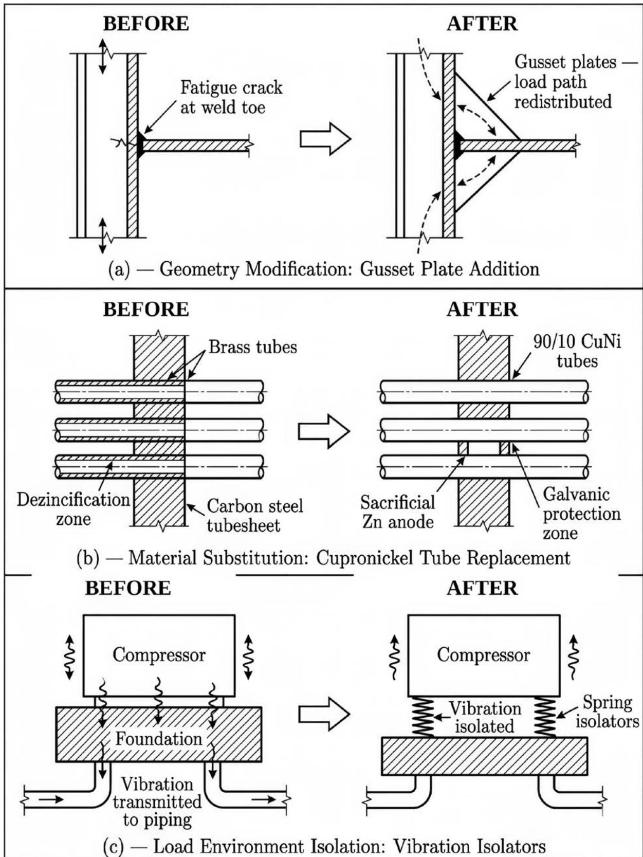
Fig. 1. Engineering schematics of three structural interventions: (a) gusset plate addition to pump support frame T-joint; (b) cupronickel tube replacement with sacrificial anode protection in seawater cooler; (c) spring vibration isolator installation on compressor foundation
