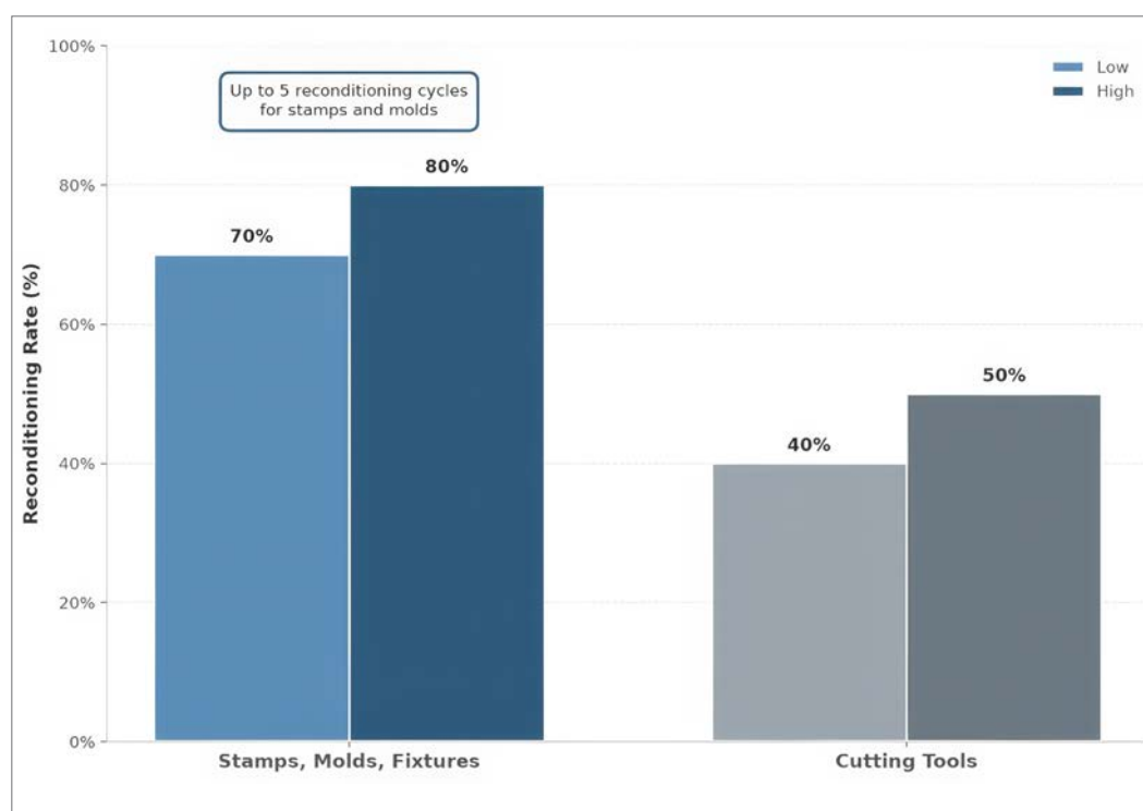
Fig. 3. Comparison of reconditioning rates by tooling category
