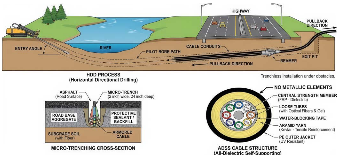
Fig. 4. Engineering process diagrams
