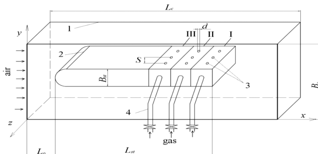
Fig. 1. Scheme of the module of the burner device of the stabilizer type with a three-row fuel gas supply: 1 — flat channel; 2 — flame stabilizer; 3 — gas supply holes; I, II, III — gas supply sections with different values of the relative pitch of the holes, corresponding to different values of the excess air coefficient
