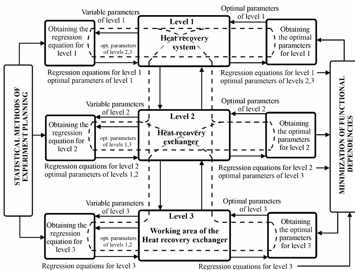
Fig. 1. Block diagram of multilevel optimization of heat recovery system designed for heating return water from boiler houses (the dotted line indicates a recursive bypass scheme for optimization levels)
