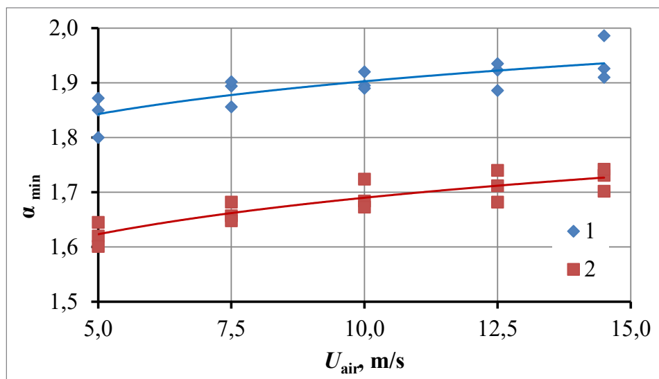
Fig. 3. Experimental dependence of the excess air coefficient \alpha_{\min} at a “rich” breakdown on the air velocity at the inlet to the burner device for different values of the distance from the gas supply openings to the breakdown edge of the flame stabilizer L_1 : 1 — L_1 = 0.015 m; 2 — L_1 = 0.03 m
