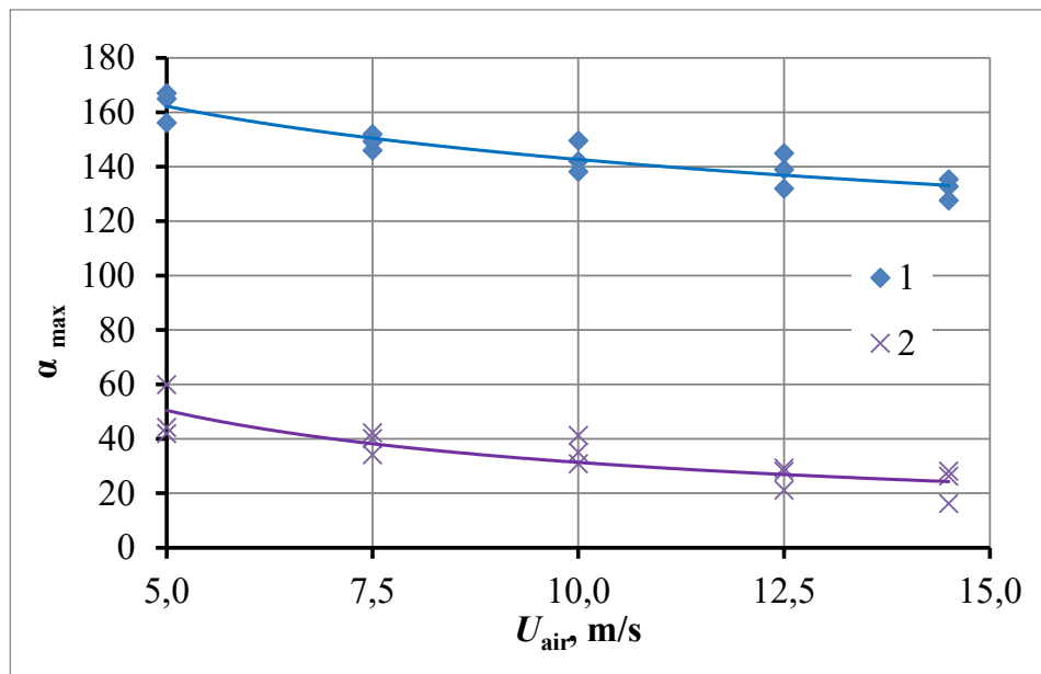
Fig. 2. Experimental dependence of the excess air coefficient \alpha_{\max} at a “lean” breakdown on the air velocity at the inlet to the burner device for different values of the relative pitch of the gas supply openings S/d : 1 — S/d = 3.2 ; 2 — S/d = 6.5
