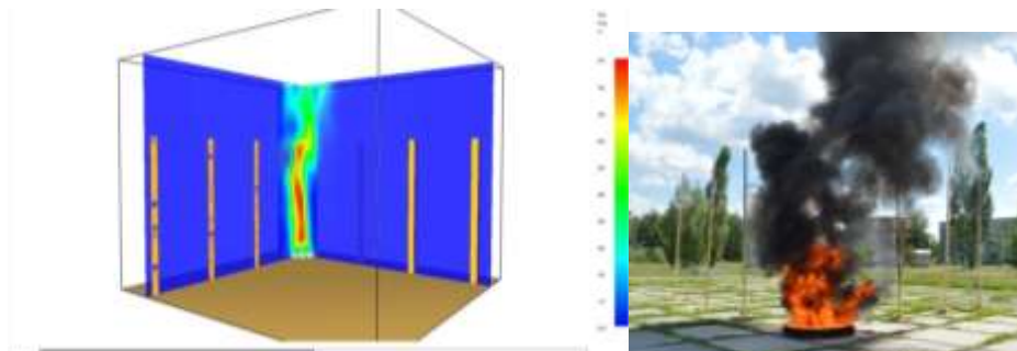
Fig. 2. Visualization of class B test fire burning at the 300 th second while performing mathematical modelling and fire test studies
