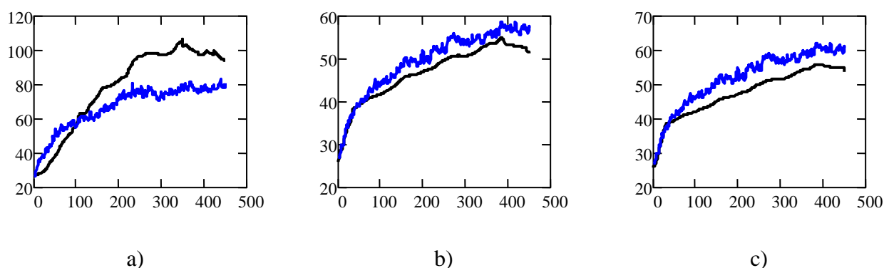
Fig. 3. Results of mathematical modelling (blue curve) and experimental studies (black curve): a) by T1 thermocouple; b) by T4 thermocouple; c) by T5 thermocouple
