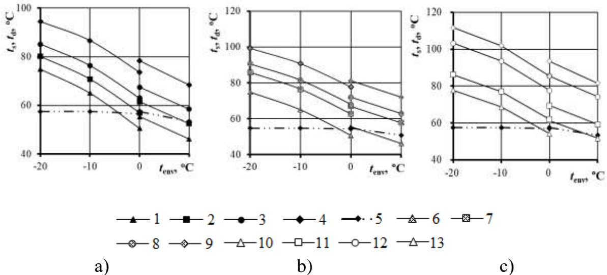
Fig. 2. Thermal characteristics of methods to prevent condensate formation in a brick chimney at the nominal temperature of exhaust-gases (after the boiler) t_{gn} = 160 °C in different modes of operation of the boiler equipment
